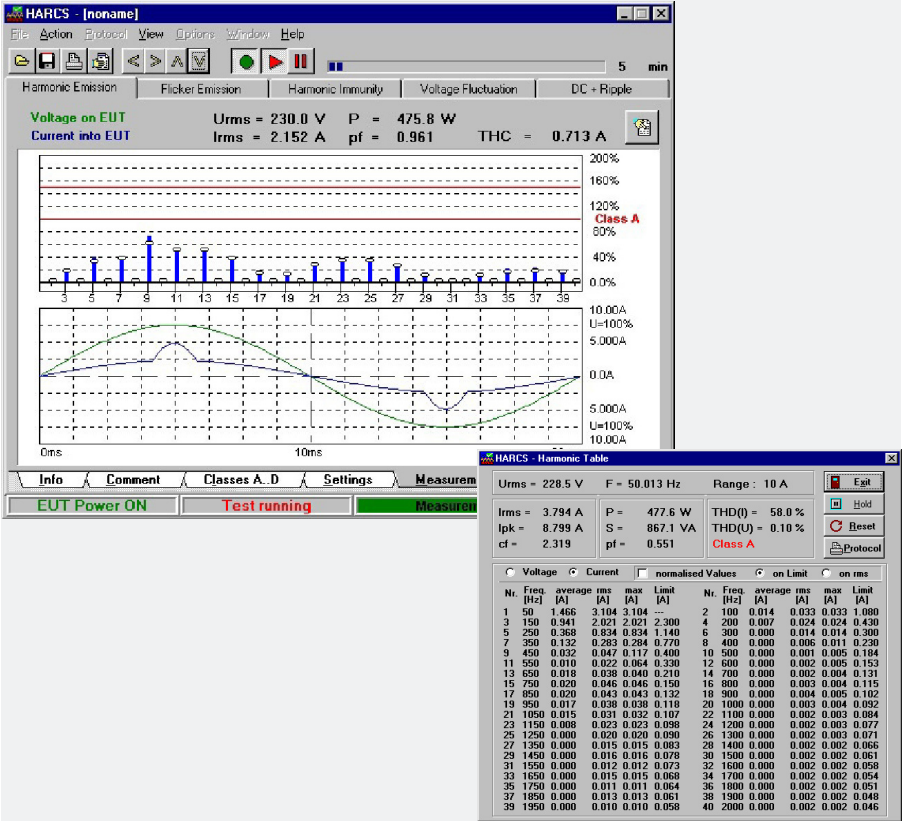
Display of single phase harmonic voltage and current (left)
